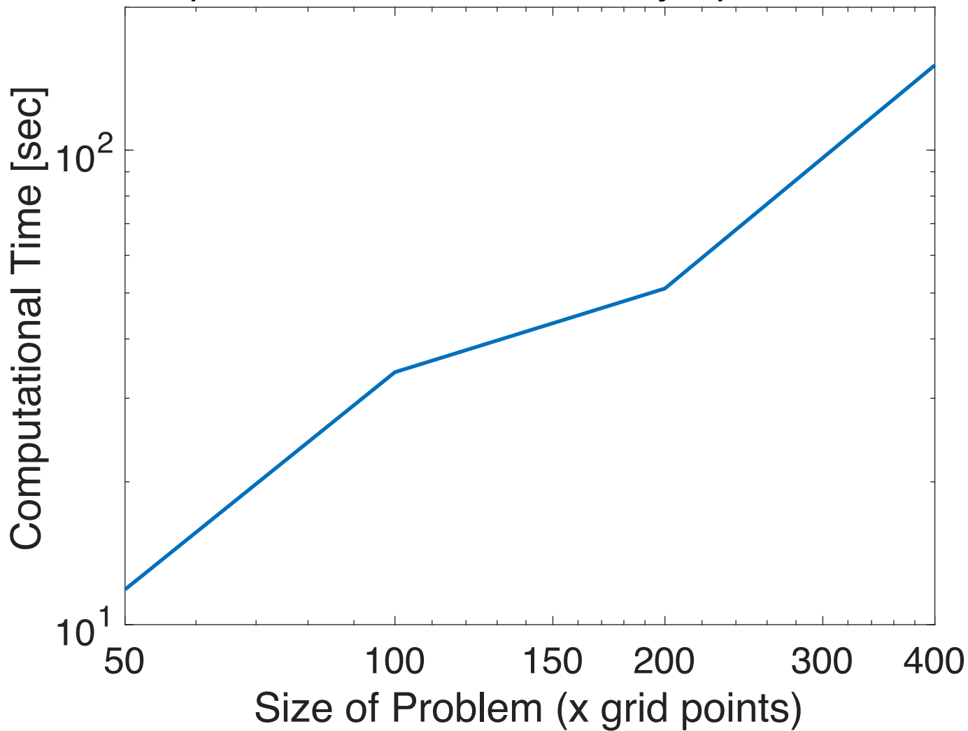
Computational Time of 3D Asymptotic Model
